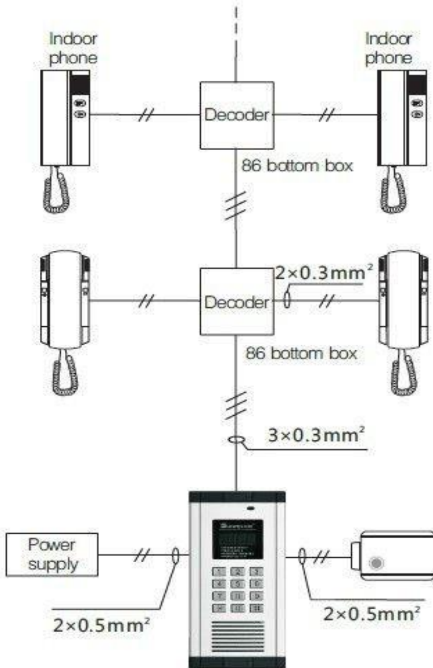
Audio doorphone system
